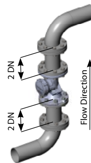
2 pipe diameters before and after elbows (90°) in vertical installations
