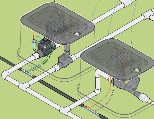
Monitoring Flow HC Flow Meter
